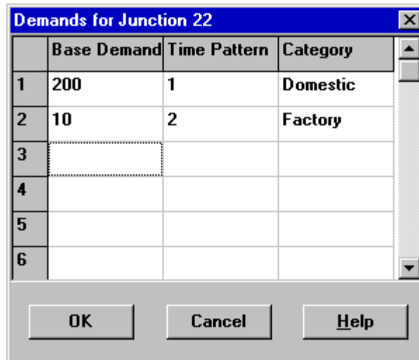
Figure 6.4 Demand Editor
